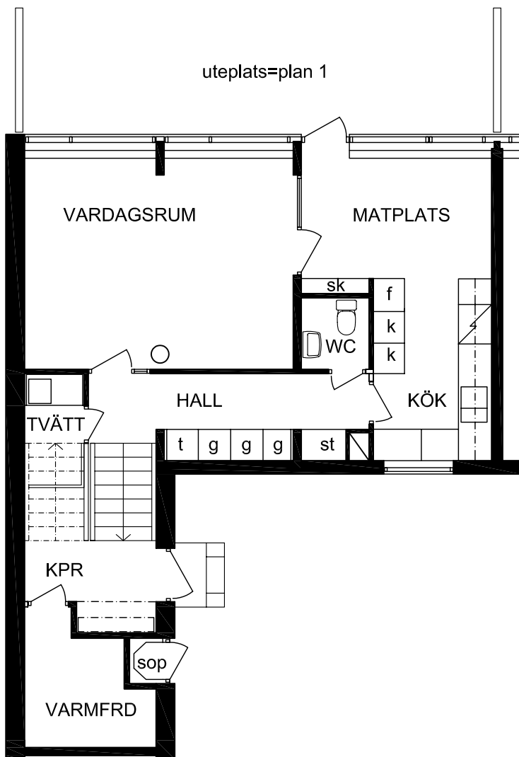
plan 1 - 58,5m 2
